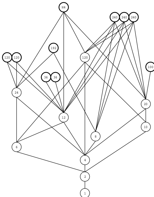
Figure 1: Classification of torus points according to their space group symmetry. Each vertex corresponds to a Wyckoff position, i.e., a class of points whose stabilizers are conjugate subgroups of the space group of the 8D periodic structure. The order of the stabilizer is inscribed into each vertex (except for H_4 ). Incidence relations of Wyckoff positions are indicated by connecting lines (those with smaller stabilizers contain others with bigger stabilizers). A Wyckoff position consists of a space group orbit of some (rational) affine subspace, wrapped on the torus. Vertices for Wyckoff positions of dimension zero (special points) are drawn with thick lines. They are discretely embedded on the torus. Each space group orbit of special points corresponds to one circle. Circles which touch each other represent orbits of special points with the same point group symmetry.
