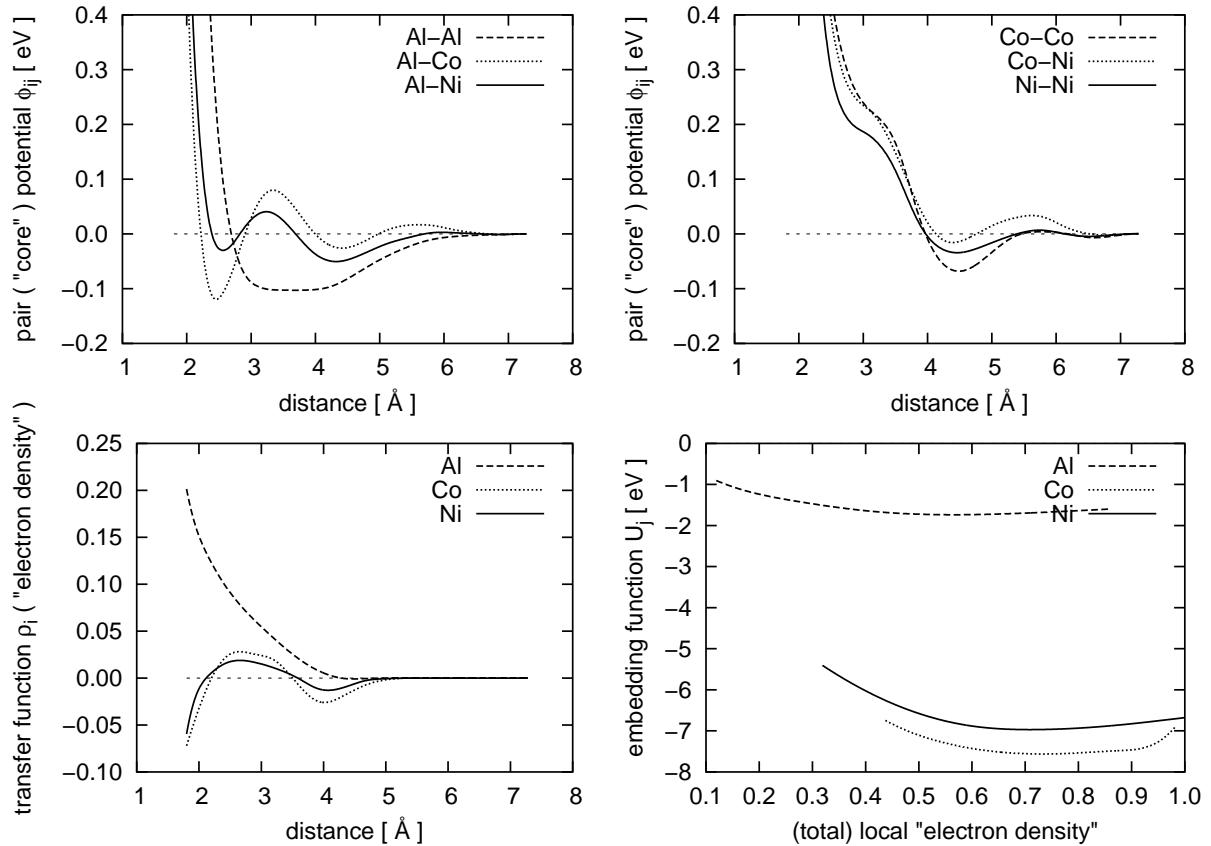
Figure 1: Potential functions for decagonal Al-Ni-Co
