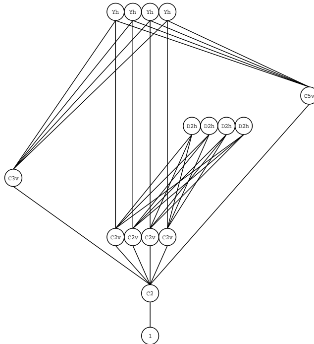
Figure 2: Structure of the Wyckoff positions of the 6D icosahedral space group F\bar{5}3\frac{2}{m} . There are special points with stabilizers Y_h = \bar{5}3m and D_{2h} = mmm (4 each), special lines with stabilizers C_{5v} = \bar{5}m , C_{3v} = \bar{3}m (1 kind each) and C_{2v} = mm (4 kinds), one kind of mirror plane, and the general position. Connections in the graph indicate incidence relations.
