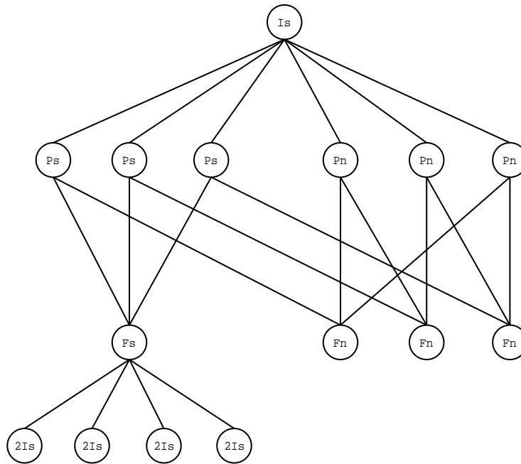
Figure 1: Part of the subgroup lattice of I\bar{5}\bar{3}\frac{2}{m} (class-equal subgroups only). A vertex label Ls means a symmorphic space group of type L\bar{5}\bar{3}\frac{2}{m} , a label Ln a non-symmorphic space group of type L\bar{5}\bar{3}\frac{2}{q} , where the lattice L is either I , P or F . 2I denotes the I lattice scaled by a factor 2. For the I lattice there exists only a symmorphic space group.
